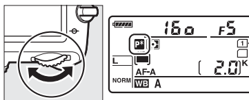
Disco de controlo principal
